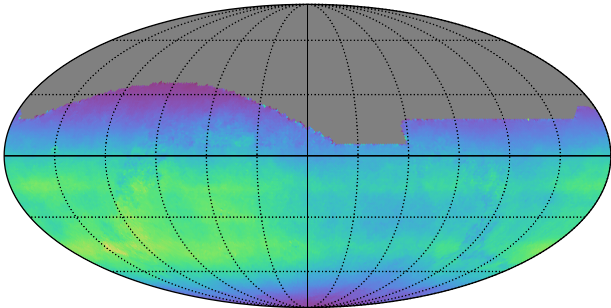
ddf_acor_sf15_lsf40_lsr20_v3.4_10yrs All sky all bands: Normalized Teff
