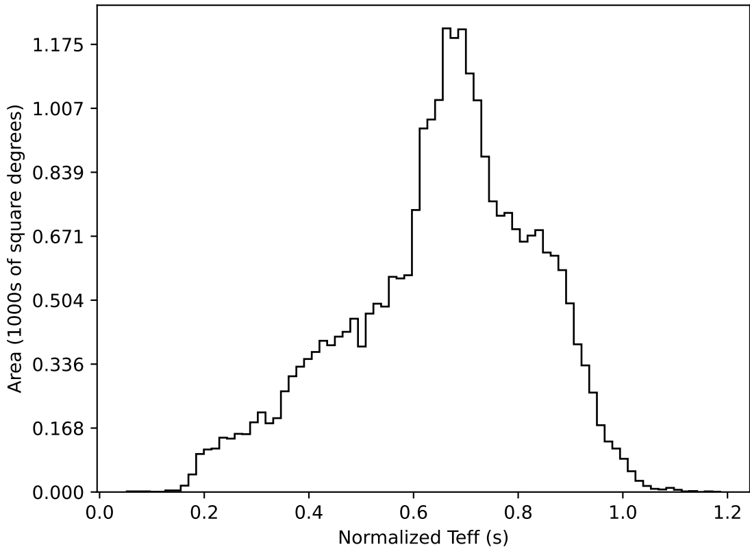
ddf_acor_sf15_lsf40_lsr20_v3.4_10yrs All sky all bands: Normalized Teff
