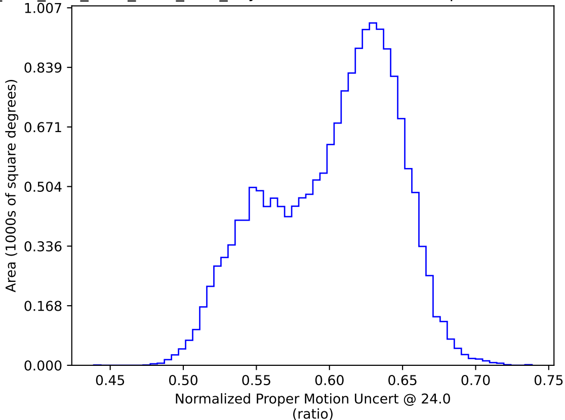
ddf_acor_sf15_lsf40_lsr20_v3.4_10yrs WFD: Normalized Proper Motion Uncert @ 24.0
