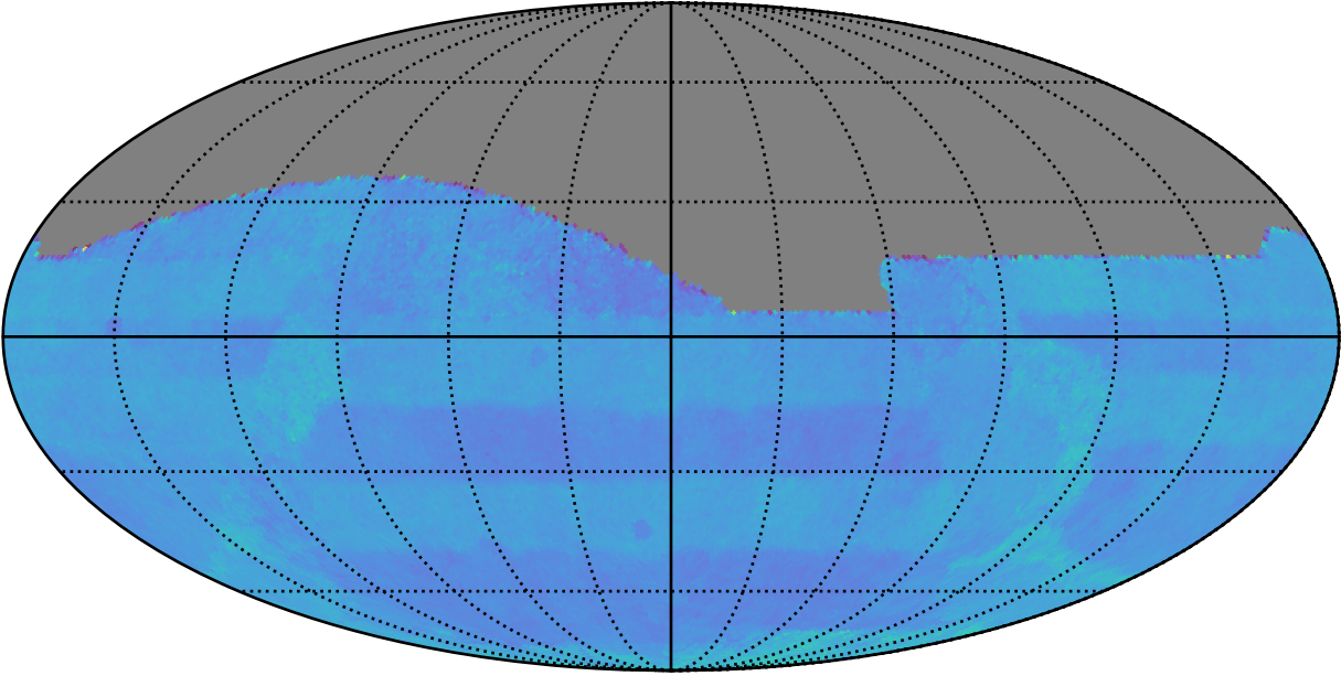
ddf_acor_sf15_lsf40_lsr20_v3.4_10yrs All sky: Normalized Proper Motion Uncert @ 24.0
