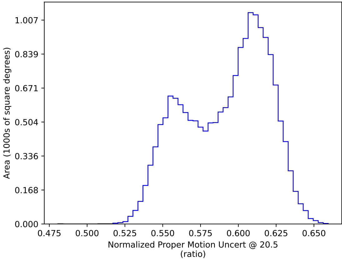
ddf_acor_sf15_lsf40_lsr20_v3.4_10yrs WFD: Normalized Proper Motion Uncert @ 20.5
