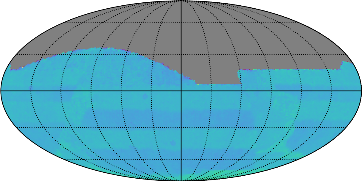
ddf_acor_sf15_lsf40_lsr20_v3.4_10yrs All sky: Normalized Proper Motion Uncert @ 20.5
