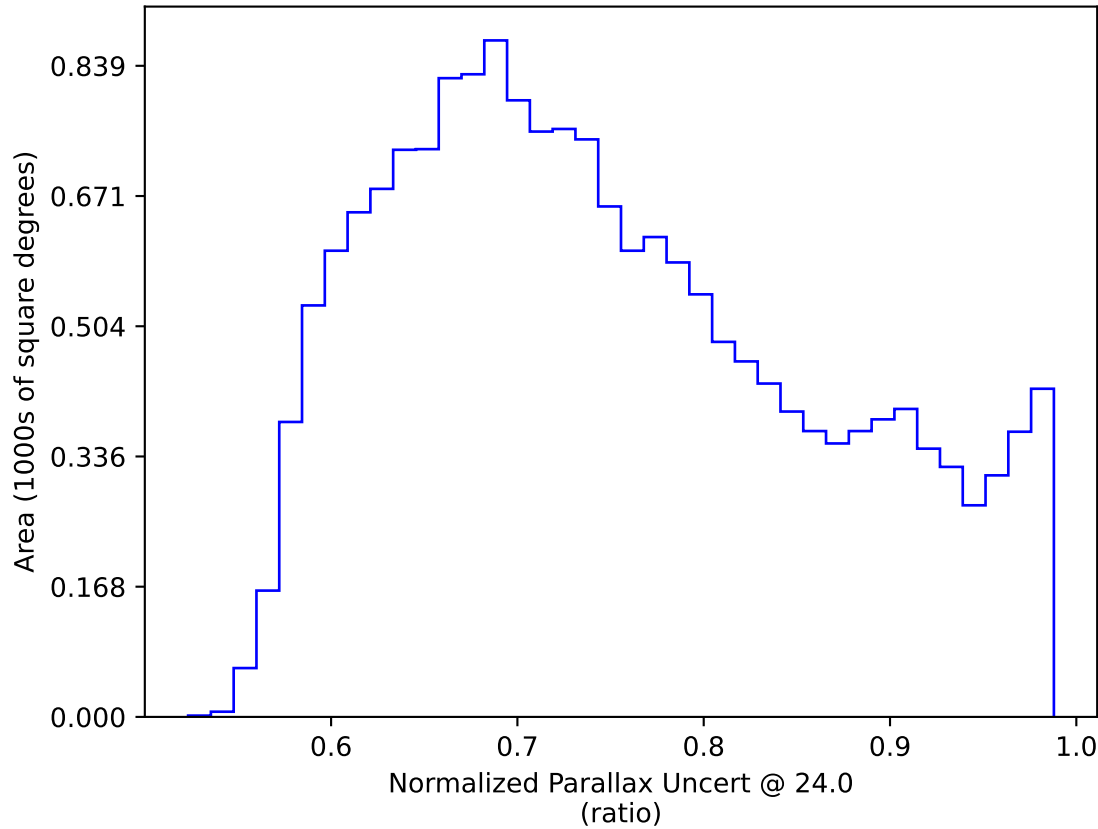
ddf_acor_sf15_ls40_lsr20_v3.4_10yrs WFD: Normalized Parallax Uncert @ 24.0
