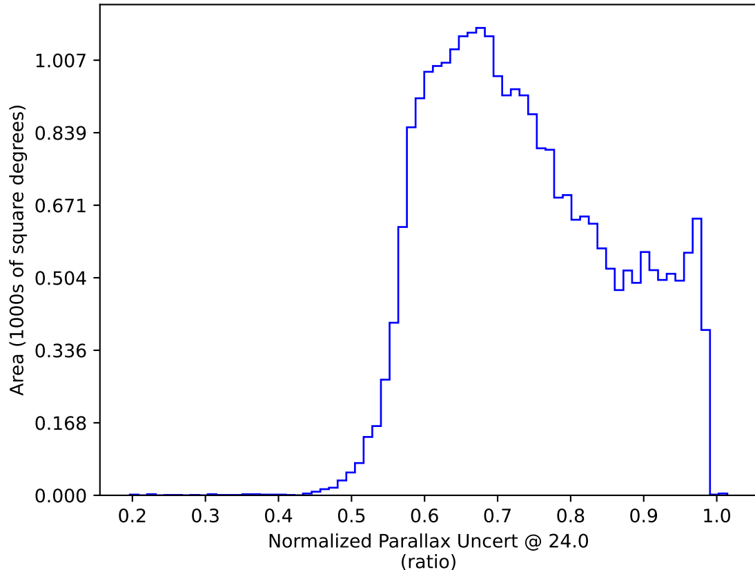
ddf_acor_sf15_lsf40_lsr20_v3.4_10yrs All sky: Normalized Parallax Uncert @ 24.0
