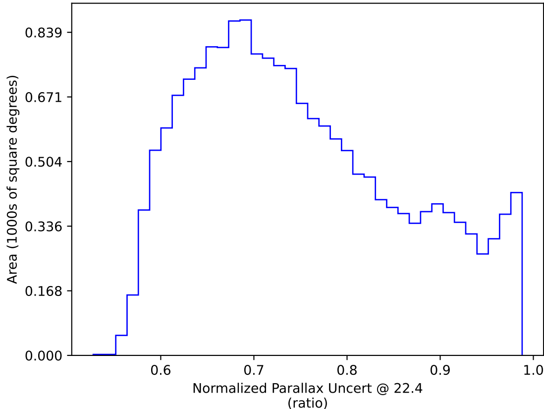
ddf_acor_sf15_lsf40_lsr20_v3.4_10yrs WFD: Normalized Parallax Uncert @ 22.4
