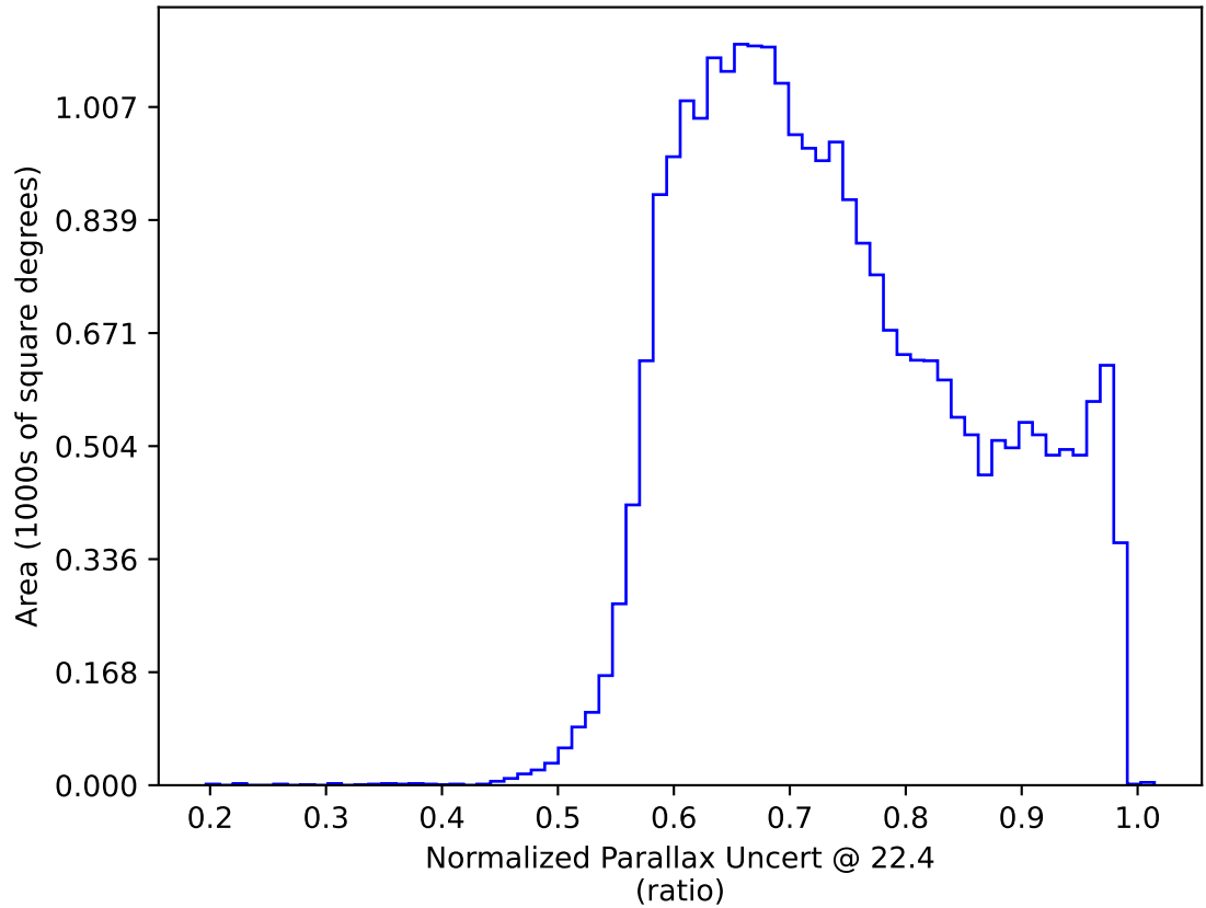
ddf_acor_sf15_lsf40_lsr20_v3.4_10yrs All sky: Normalized Parallax Uncert @ 22.4
