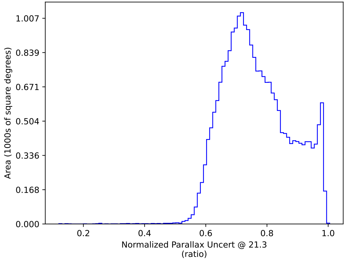
ddf_acor_sf15_lsf40_lsr20_v3.4_10yrs All sky y band only: Normalized Parallax Uncert @ 21.3
