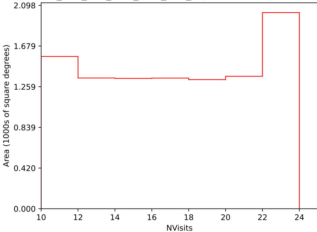
ddf_acor_sf15_lsf40_lsr20_v3.4_10yrs Yr 3-4 i band: NVisits
