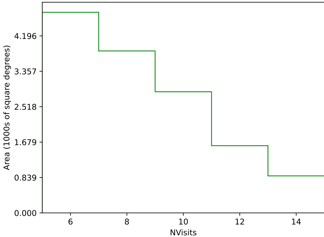
ddf_acor_sf15_lsf40_lsr20_v3.4_10yrs Yr 3-4 g band: NVisits
