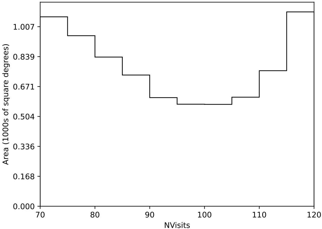
ddf_acor_sf15_lsf40_lsr20_v3.4_10yrs Yr 3-4 all bands: NVisits
