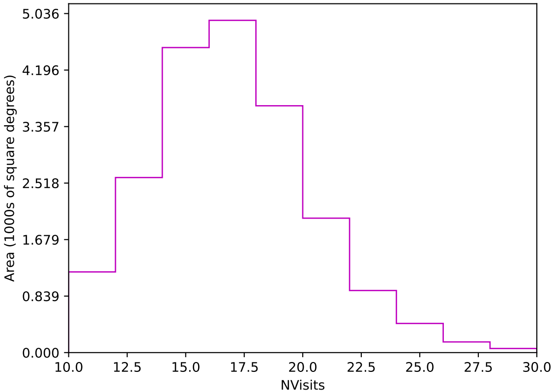
ddf_acor_sf15_lsf40_lsr20_v3.4_10yrs Yr 1 z band: NVisits
