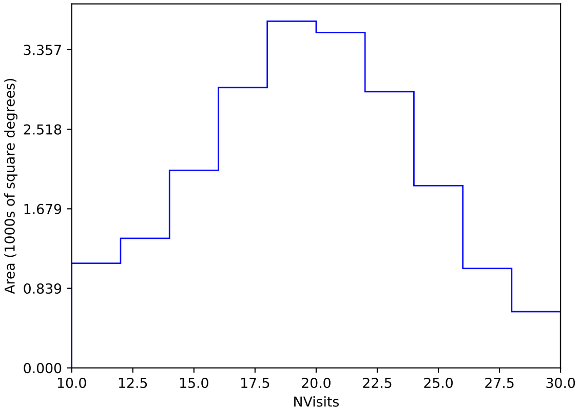
ddf_acor_sf15_lsf40_lsr20_v3.4_10yrs Yr 1 y band: NVisits
