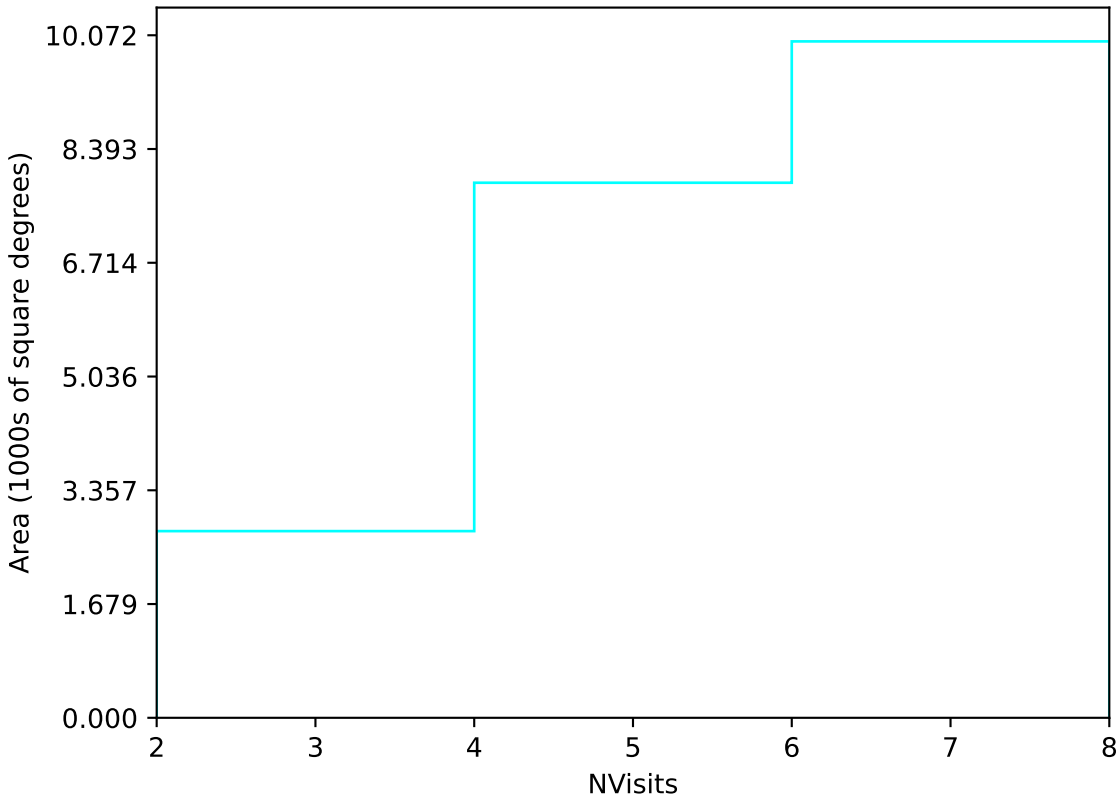
ddf_acor_sf15_lsf40_lsr20_v3.4_10yrs Yr 1 u band: NVisits
