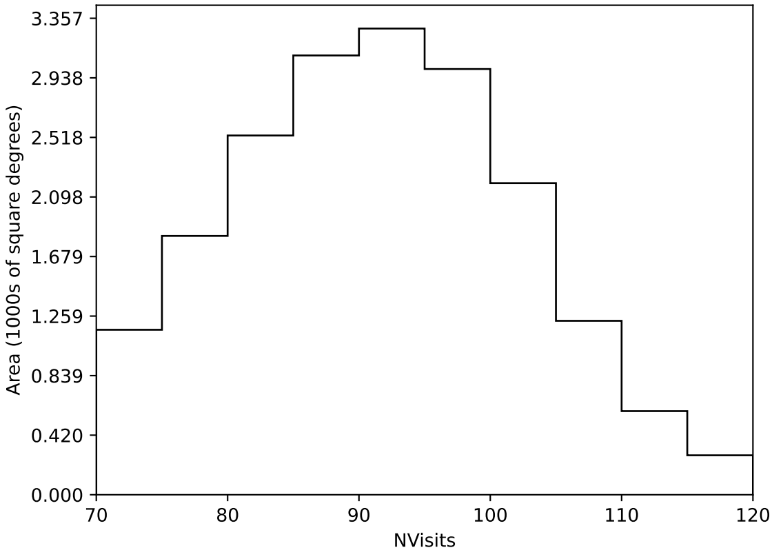
ddf_acor_sf15_lsf40_lsr20_v3.4_10yrs Yr 1 all bands: NVisits
