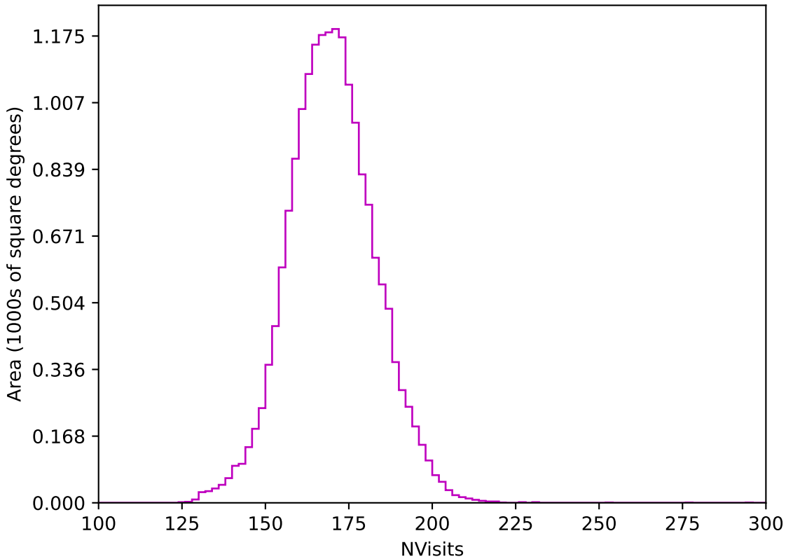
ddf_acor_sf15_lsf40_lsr20_v3.4_10yrs WFD z band: NVisits
