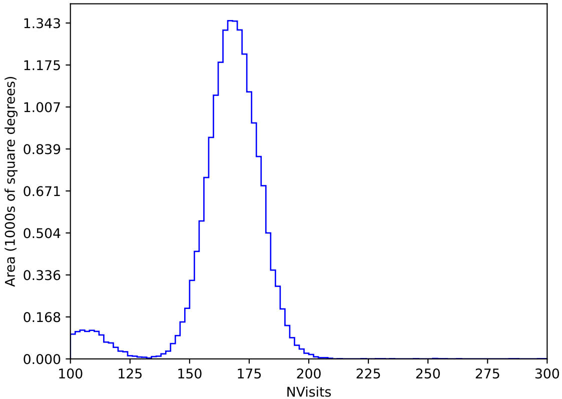
ddf_acor_sf15_lsf40_lsr20_v3.4_10yrs WFD y band: NVisits
