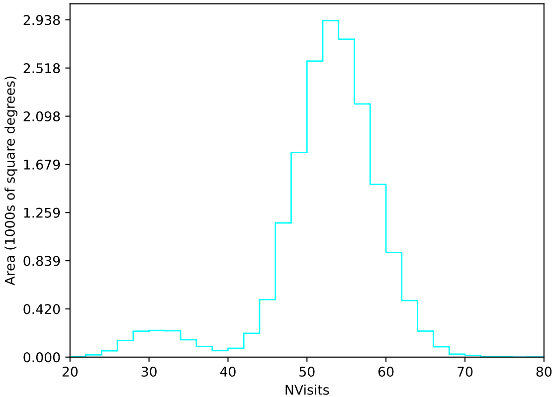
ddf_acor_sf15_lsf40_lsr20_v3.4_10yrs WFD u band: NVisits
