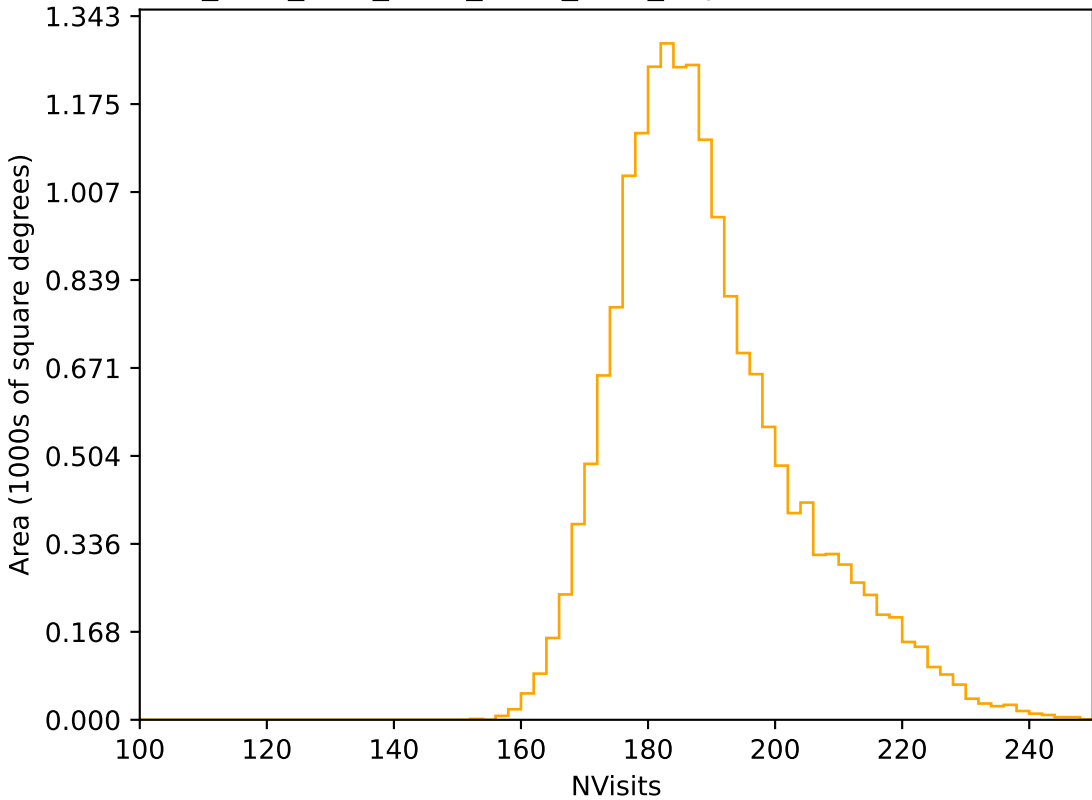
ddf_acor_sf15_lsf40_lsr20_v3.4_10yrs WFD r band: NVisits
