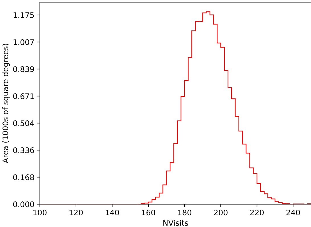
ddf_acor_sf15_lsf40_lsr20_v3.4_10yrs WFD i band: NVisits
