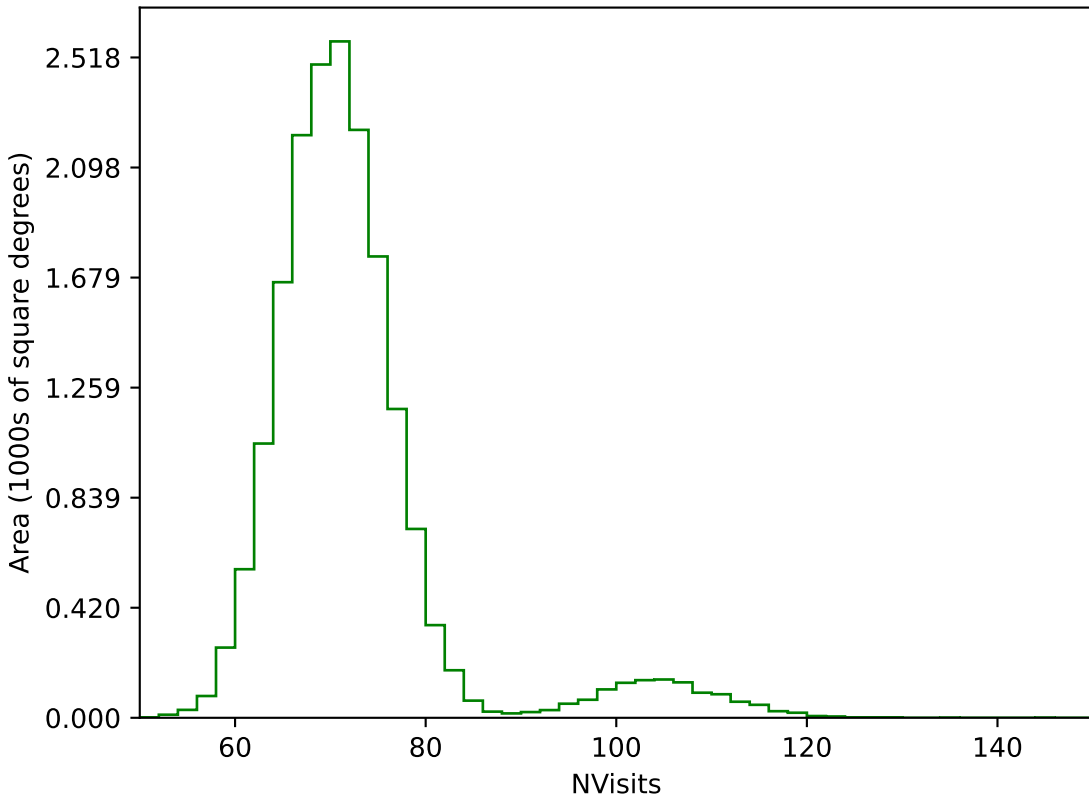
ddf_acor_sf15_lsf40_lsr20_v3.4_10yrs WFD g band: NVisits
