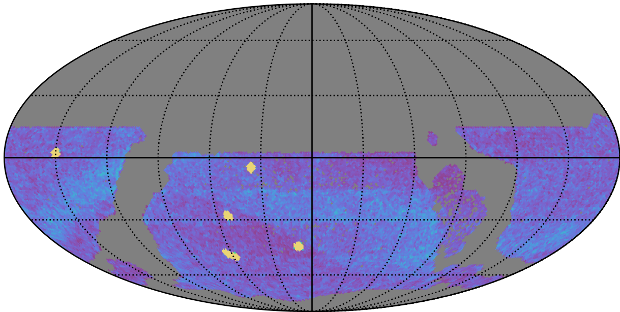
ddf_acor_sf15_lsf40_lsr20_v3.4_10yrs WFD all bands: NVisits
