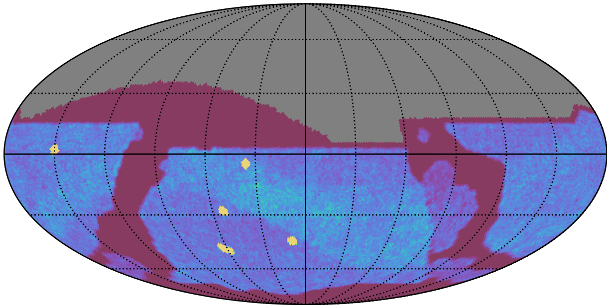
ddf_acor_sf15_lsf40_lsr20_v3.4_10yrs All sky z band: NVisits
