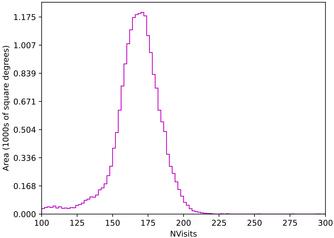
ddf_acor_sf15_ls40_lsr20_v3.4_10yrs All sky z band: NVisits
