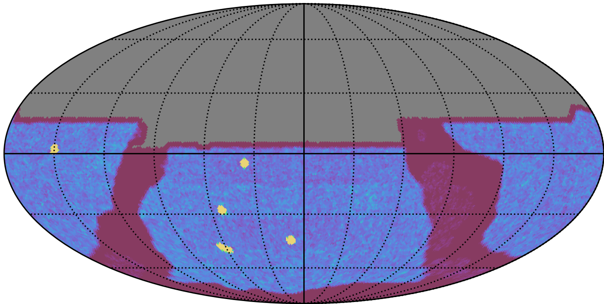
ddf_acor_sf15_lsf40_lsr20_v3.4_10yrs All sky y band: NVisits
