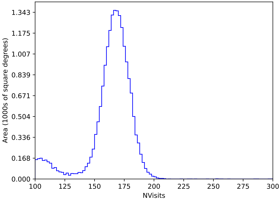
ddf_acor_sf15_lsf40_lsr20_v3.4_10yrs All sky y band: NVisits
