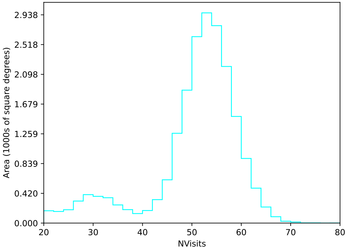
ddf_acor_sf15_ls40_lsr20_v3.4_10yrs All sky u band: NVisits
