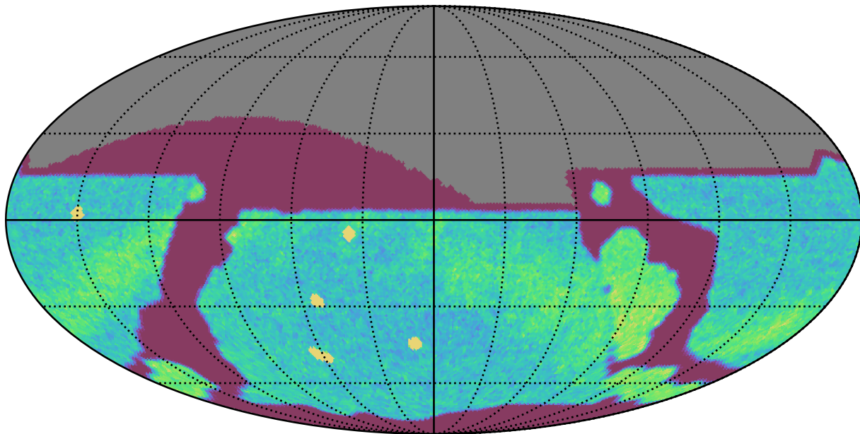
ddf_acor_sf15_lsf40_lsr20_v3.4_10yrs All sky r band: NVisits
