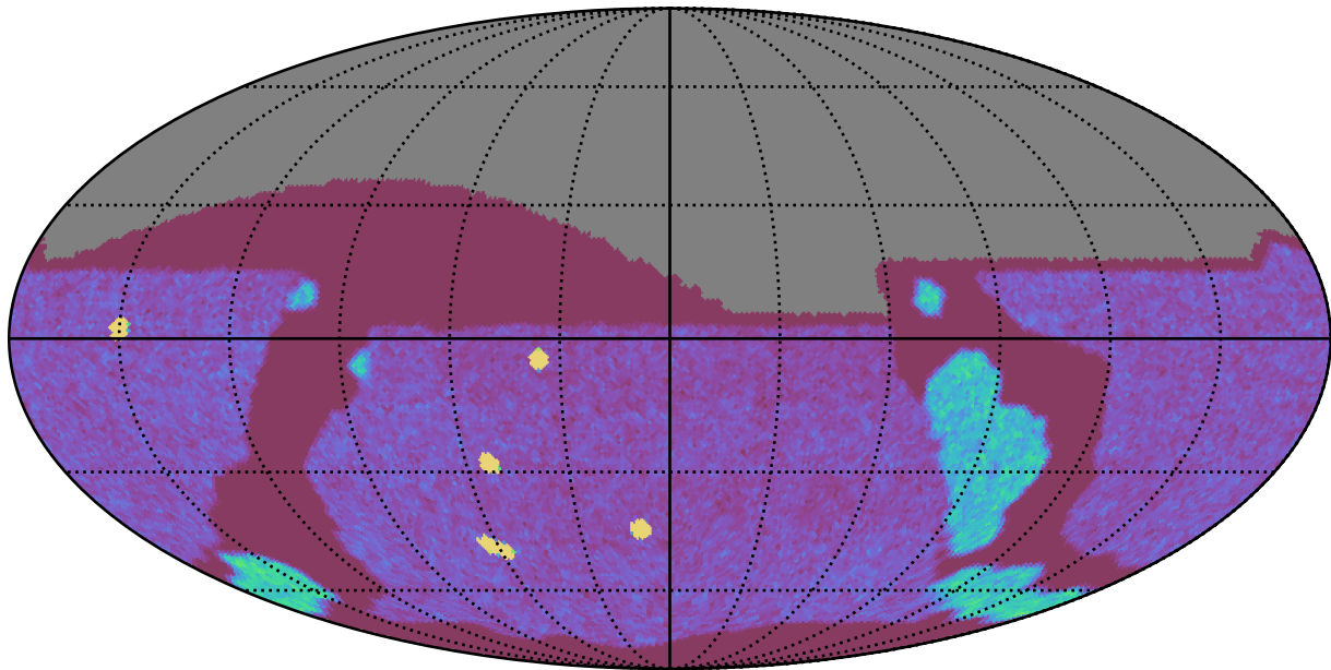
ddf_acor_sf15_lsf40_lsr20_v3.4_10yrs All sky g band: NVisits
