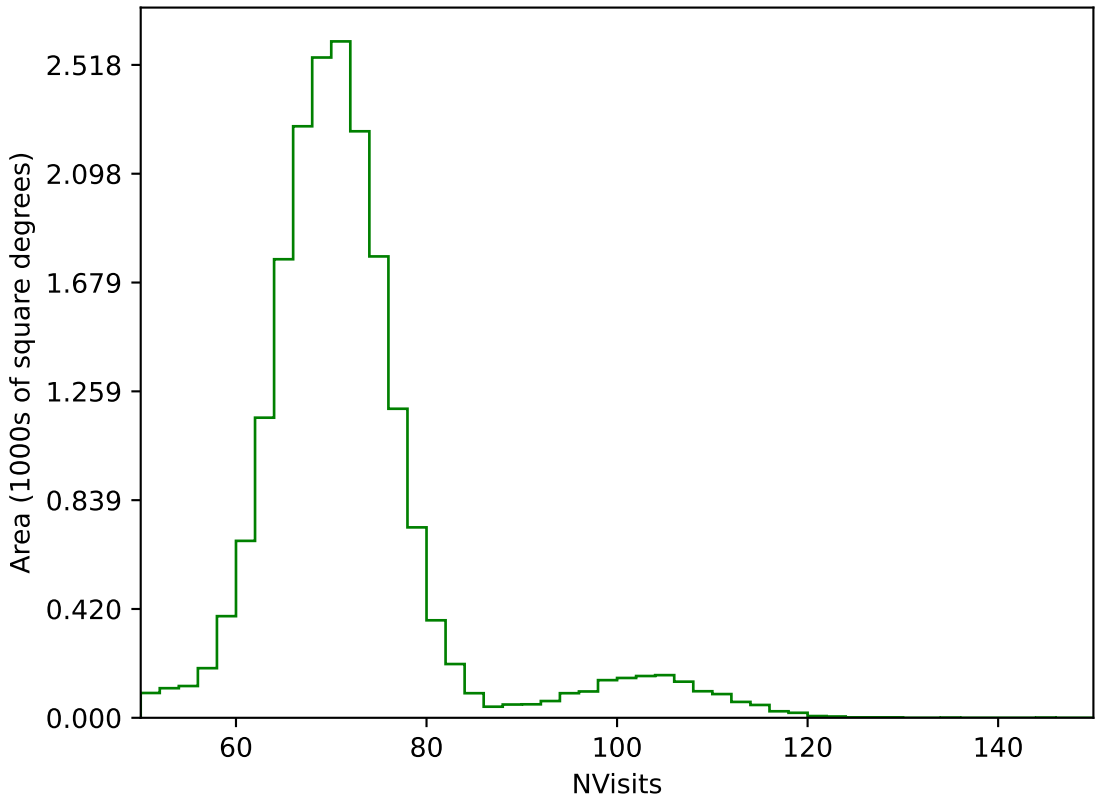
ddf_acor_sf15_lsf40_lsr20_v3.4_10yrs All sky g band: NVisits
