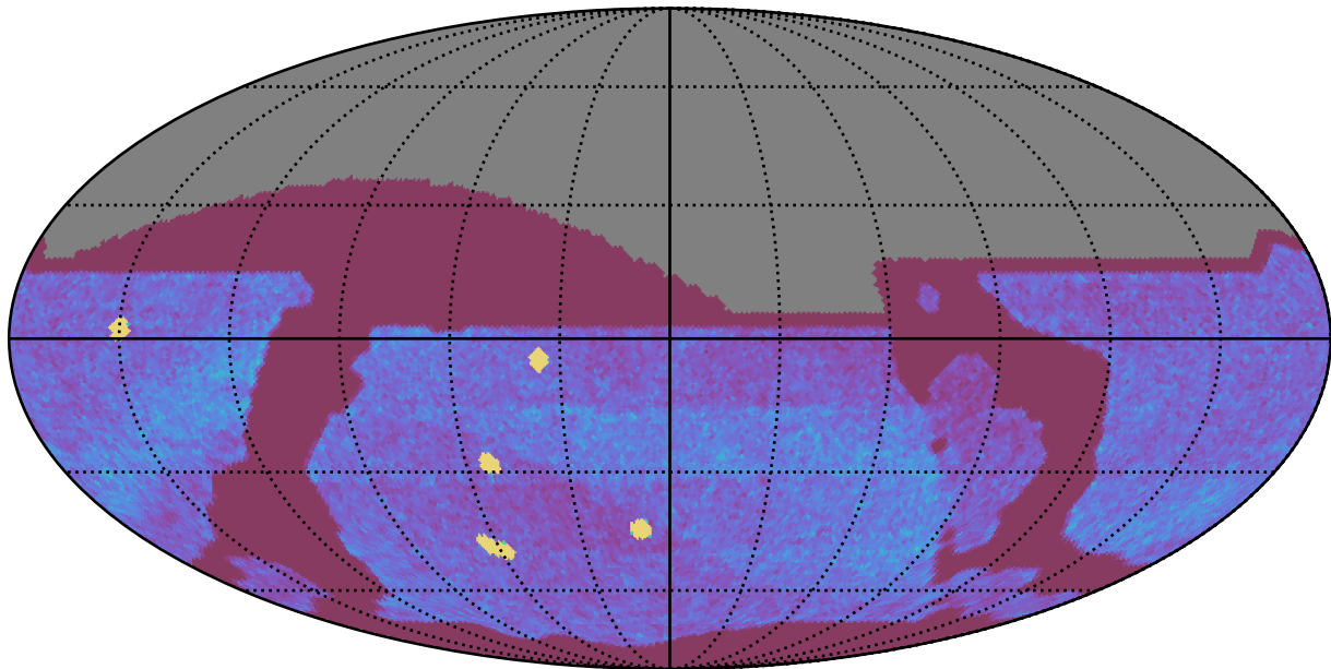
ddf_acor_sf15_lsf40_lsr20_v3.4_10yrs All sky all bands: NVisits
