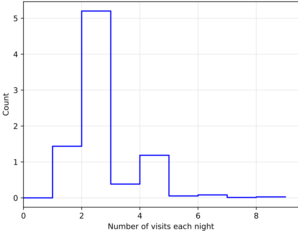
ddf_acor_sf15_lsf40_lsr20_v3.4_10yrs WFD: NVisitsPerNight 1e6
