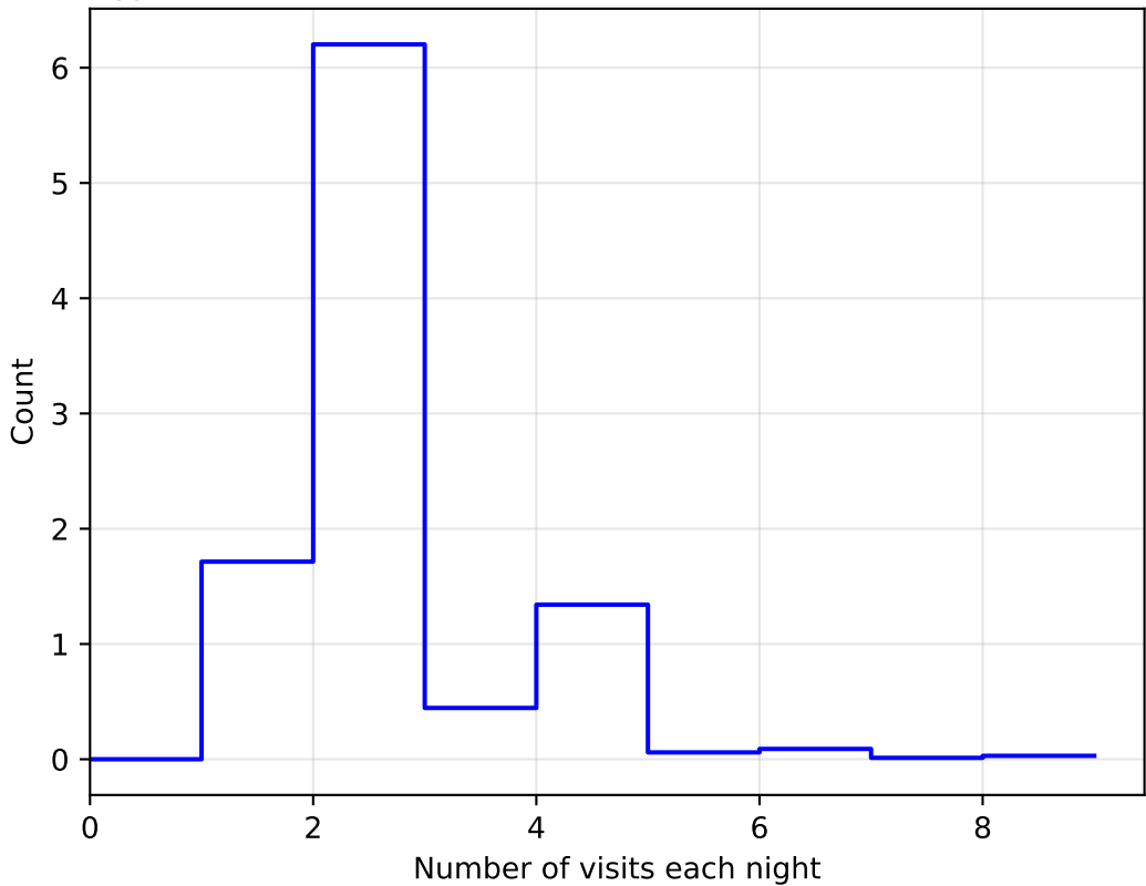
ddf_acor_sf15_lsf40_lsr20_v3.4_10yrs All sky: NVisitsPerNight 1e6
