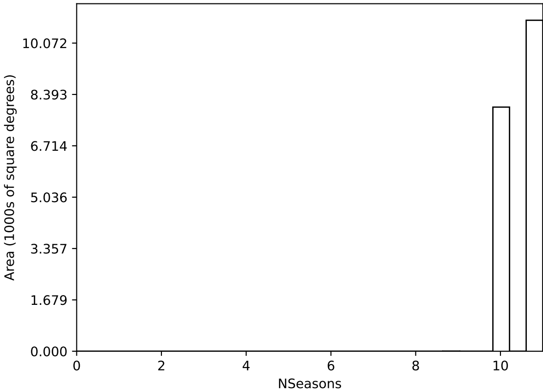
ddf_acor_sf15_lsf40_lsr20_v3.4_10yrs WFD all bands: NSeasons
