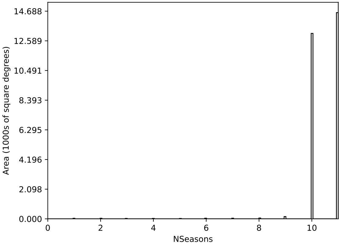
ddf_acor_sf15_lsf40_lsr20_v3.4_10yrs All sky all bands: NSeasons
