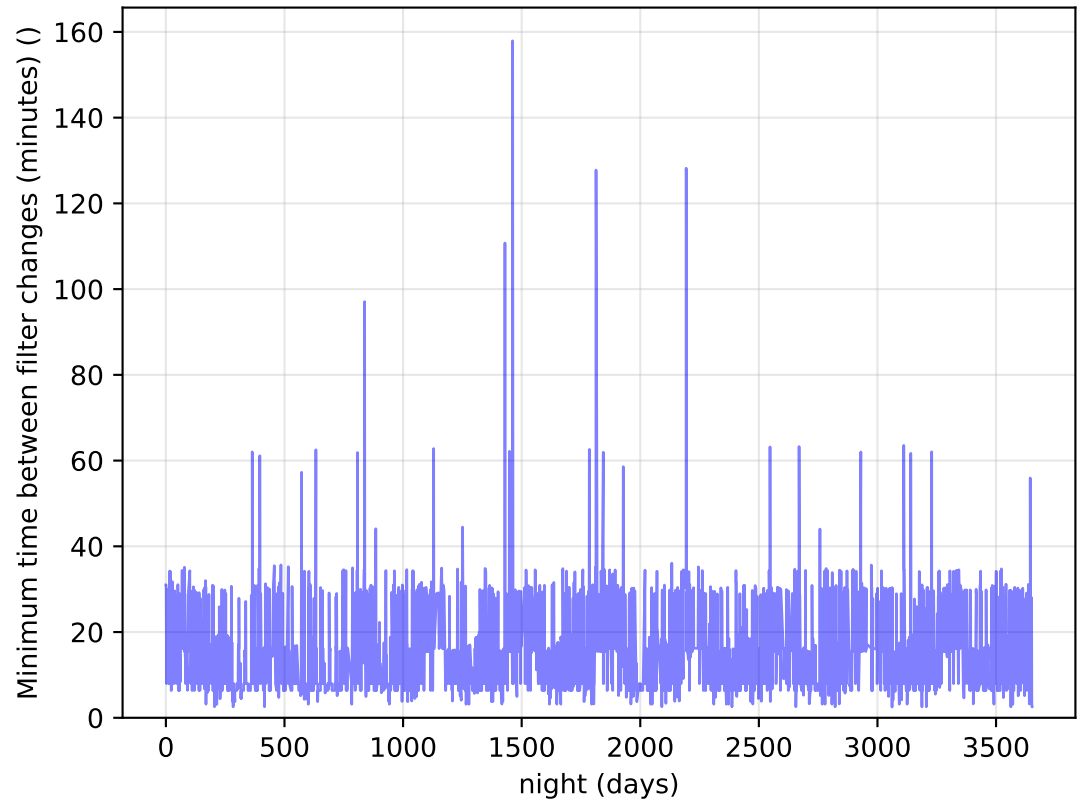
ddf_acor_sf15_Isf40_Isr20_v3.4_10yrs Per Night: Minimum time between filter changes (minutes)
