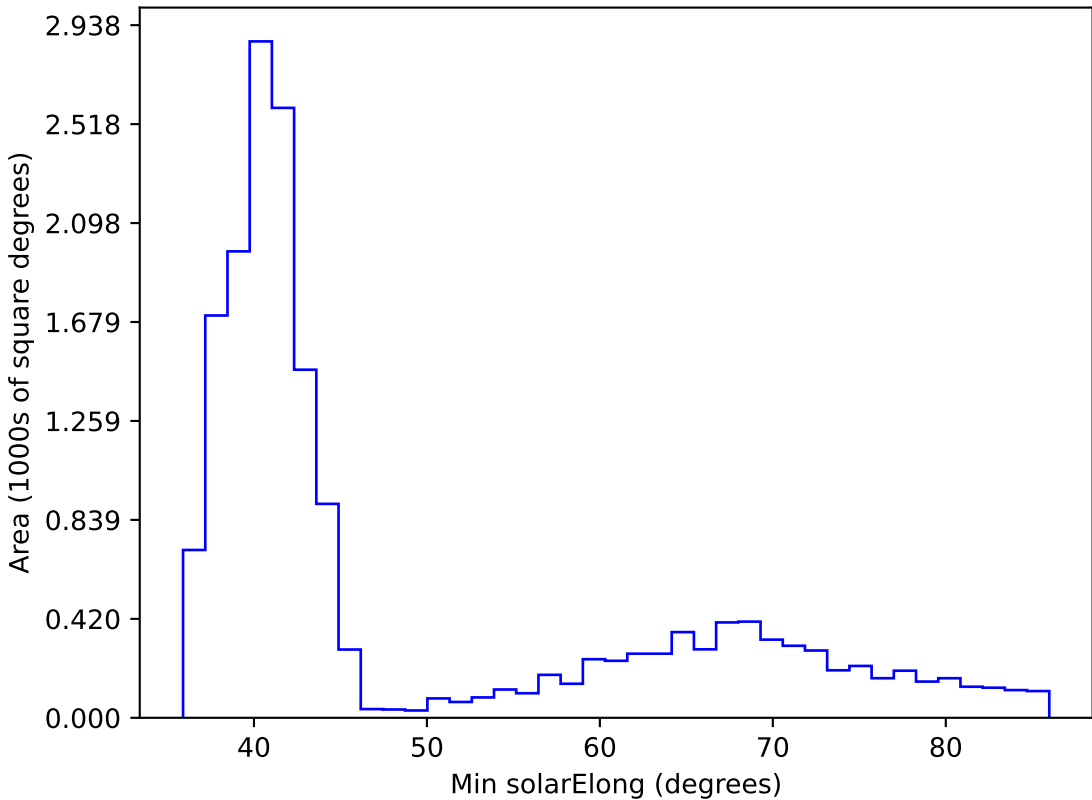
ddf_acor_sf15_lsf40_lsr20_v3.4_10yrs WFD z band: Min solarElong
