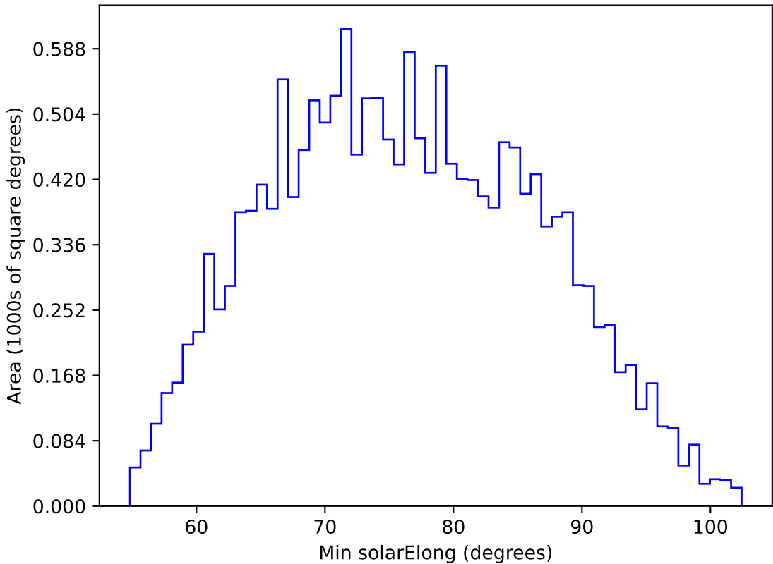
ddf_acor_sf15_lsf40_lsr20_v3.4_10yrs WFD u band: Min solarElong
