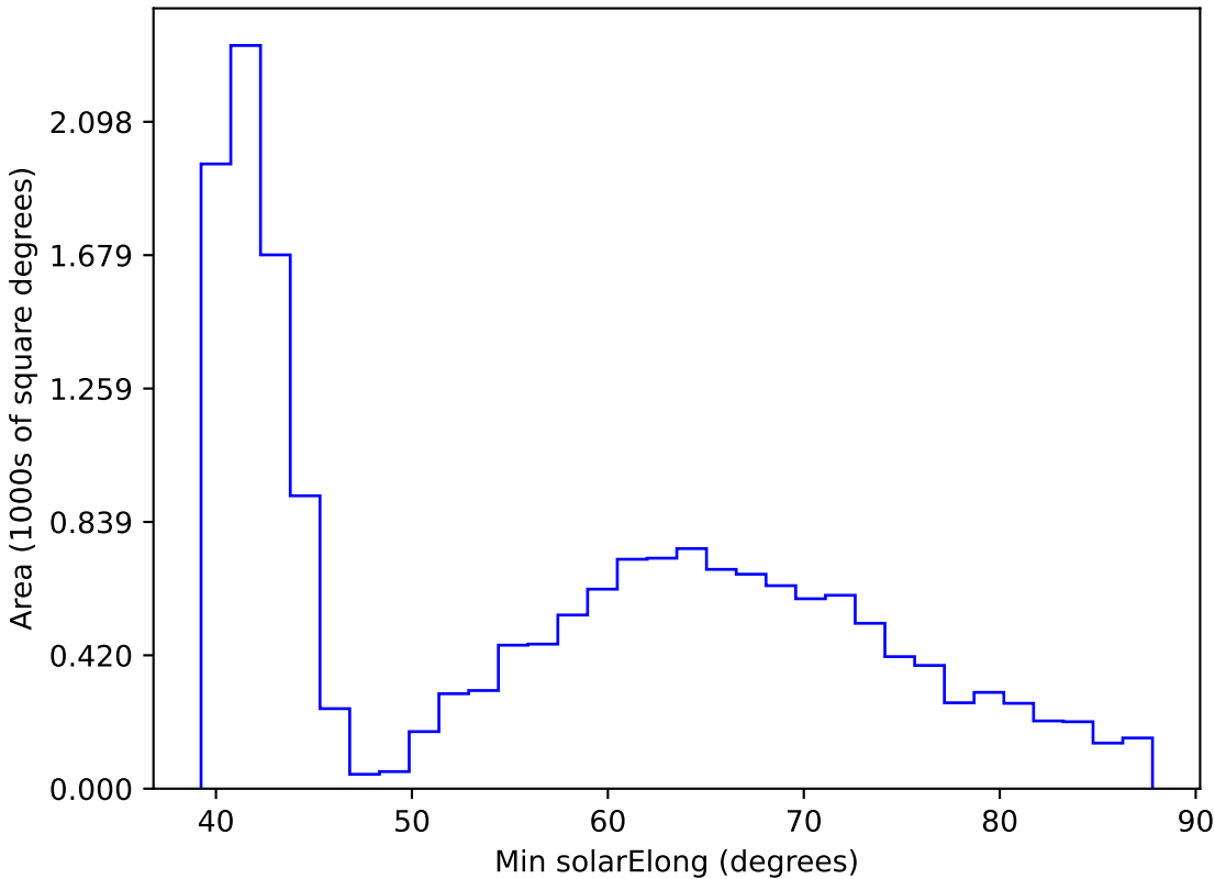
ddf_acor_sf15_lsf40_lsr20_v3.4_10yrs WFD r band: Min solarElong
