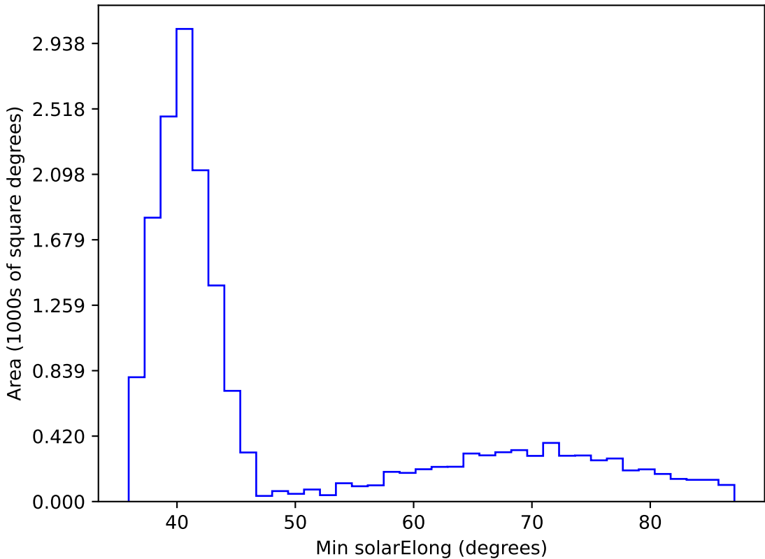
ddf_acor_sf15_lsf40_lsr20_v3.4_10yrs WFD i band: Min solarElong
