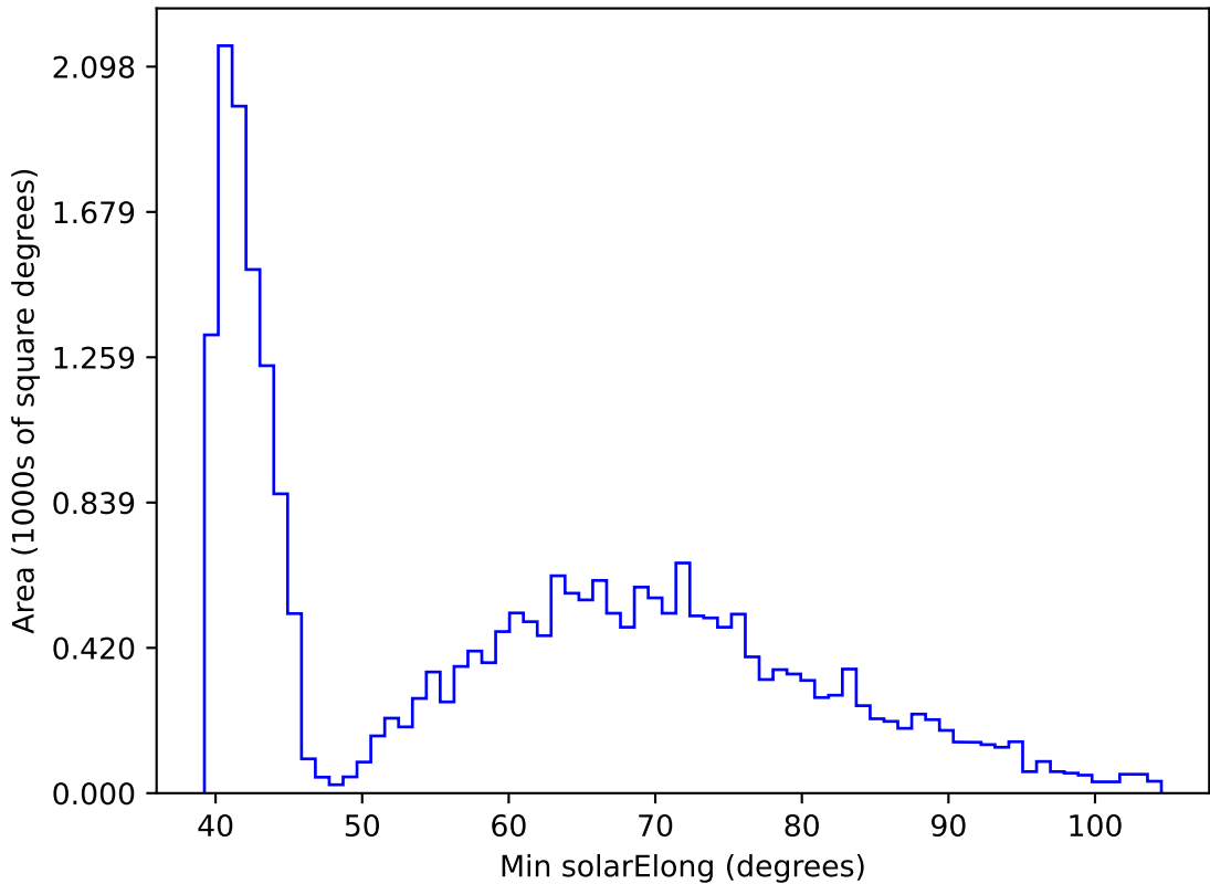
ddf_acor_sf15_ls40_lsr20_v3.4_10yrs All sky r band: Min solarElong
