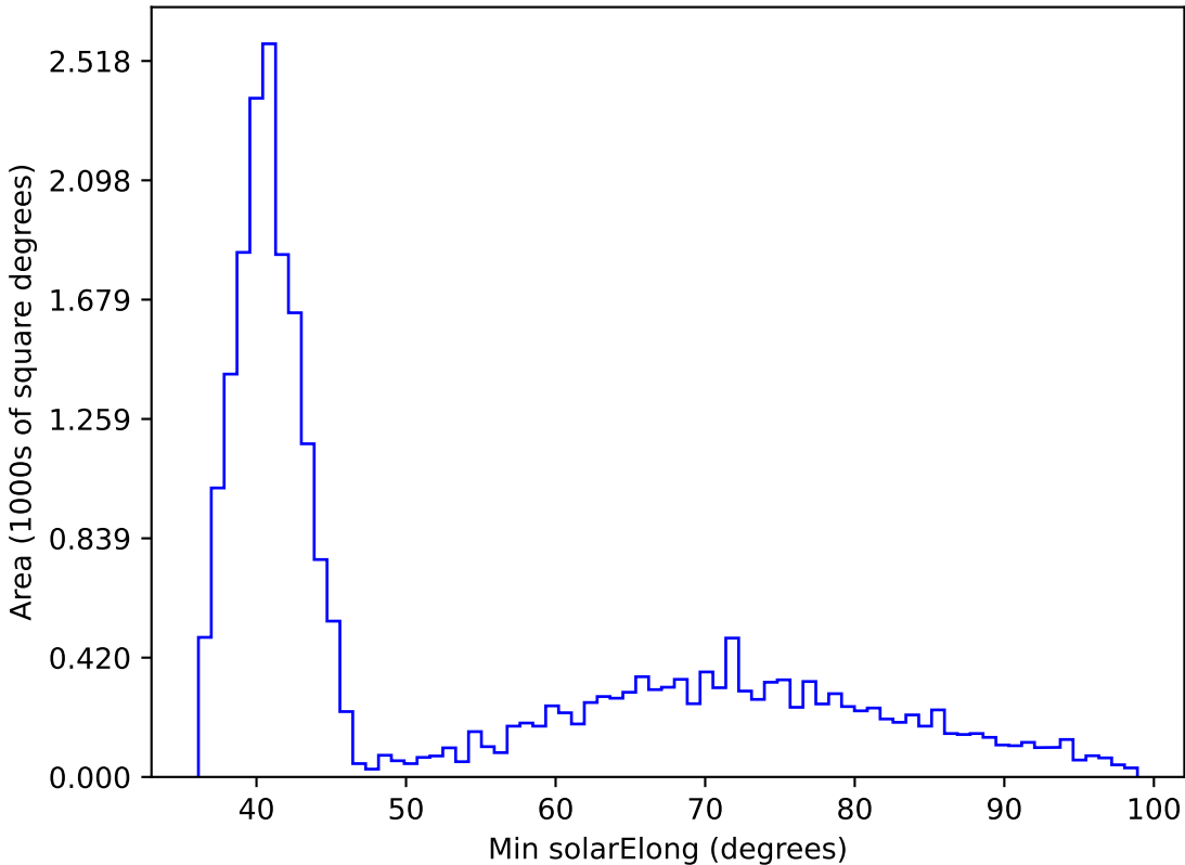
ddf_acor_sf15_lsf40_lsr20_v3.4_10yrs All sky i band: Min solarElong
