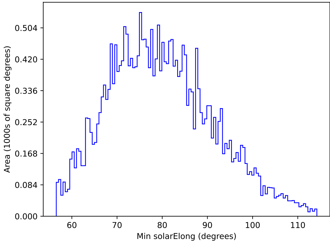
ddf_acor_sf15_lsf40_lsr20_v3.4_10yrs All sky g band: Min solarElong
