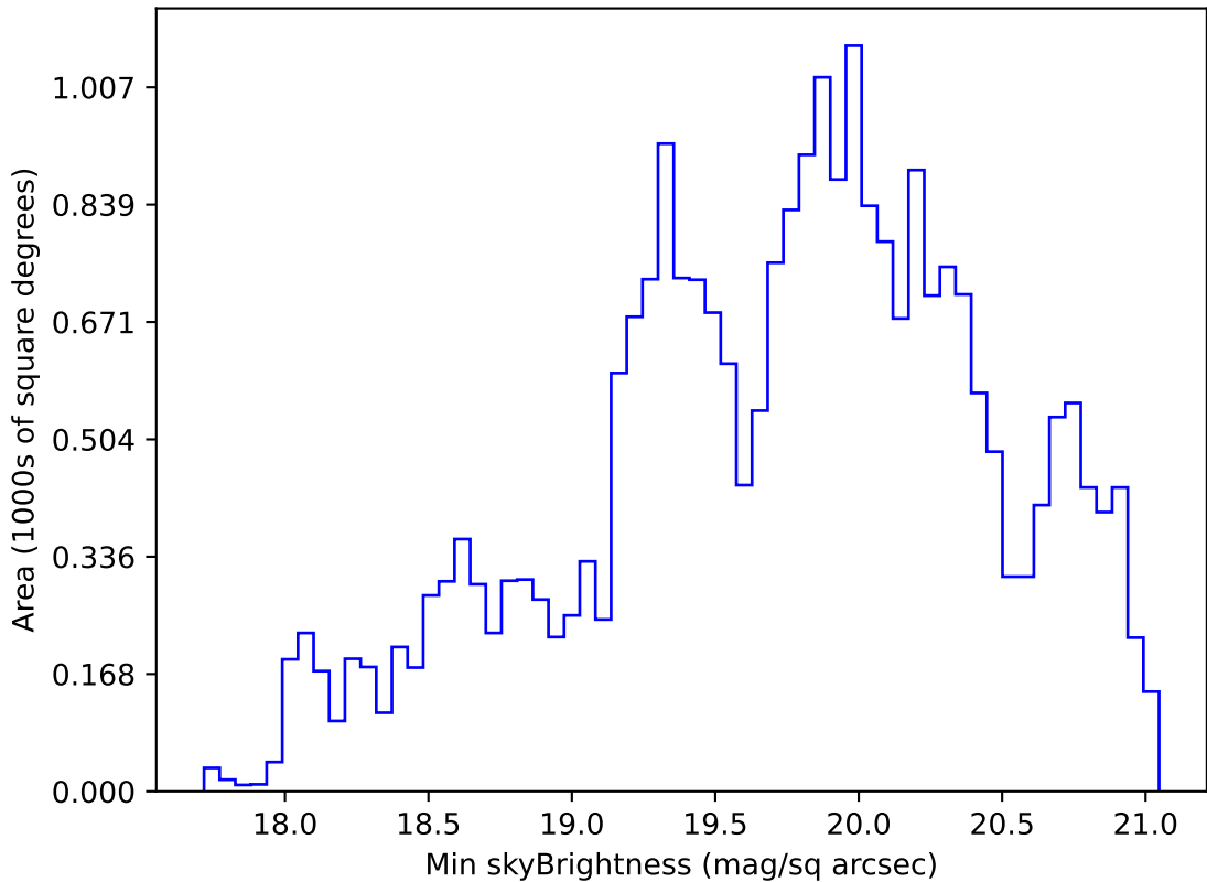
ddf_acor_sf15_lsf40_lsr20_v3.4_10yrs Yr 1 r band: Min skyBrightness
