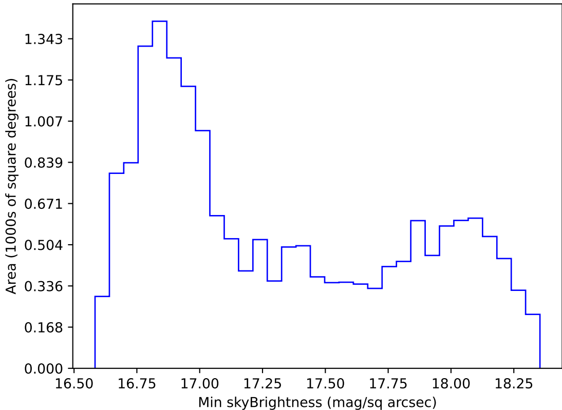
ddf_acor_sf15_lsf40_lsr20_v3.4_10yrs WFD z band: Min skyBrightness
