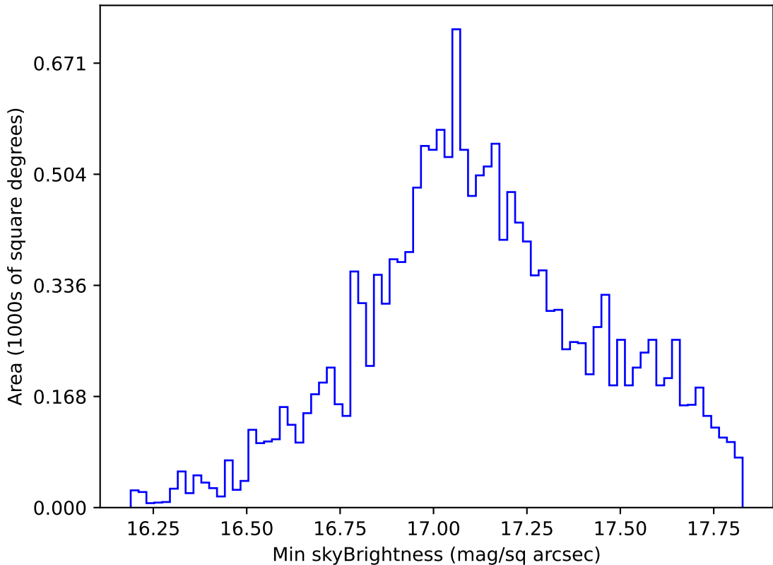
ddf_acor_sf15_lsf40_lsr20_v3.4_10yrs WFD y band: Min skyBrightness
