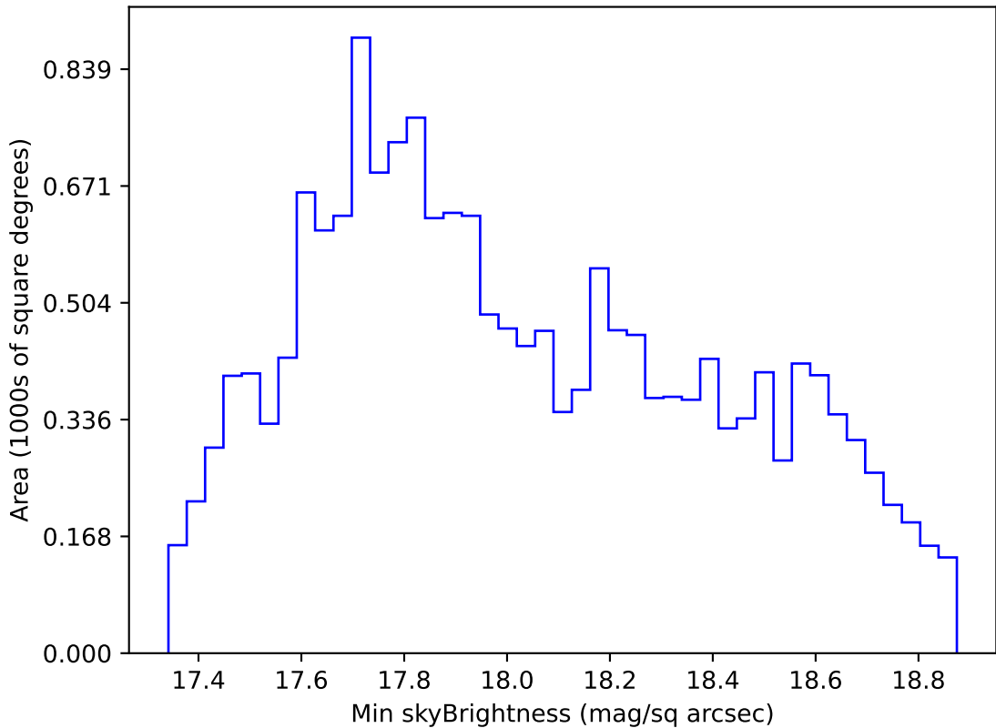
ddf_acor_sf15_lsf40_lsr20_v3.4_10yrs WFD i band: Min skyBrightness
